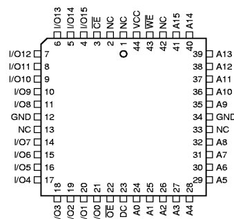
PLCC Top View
